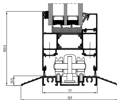
door with low-level threshold, bottom view
